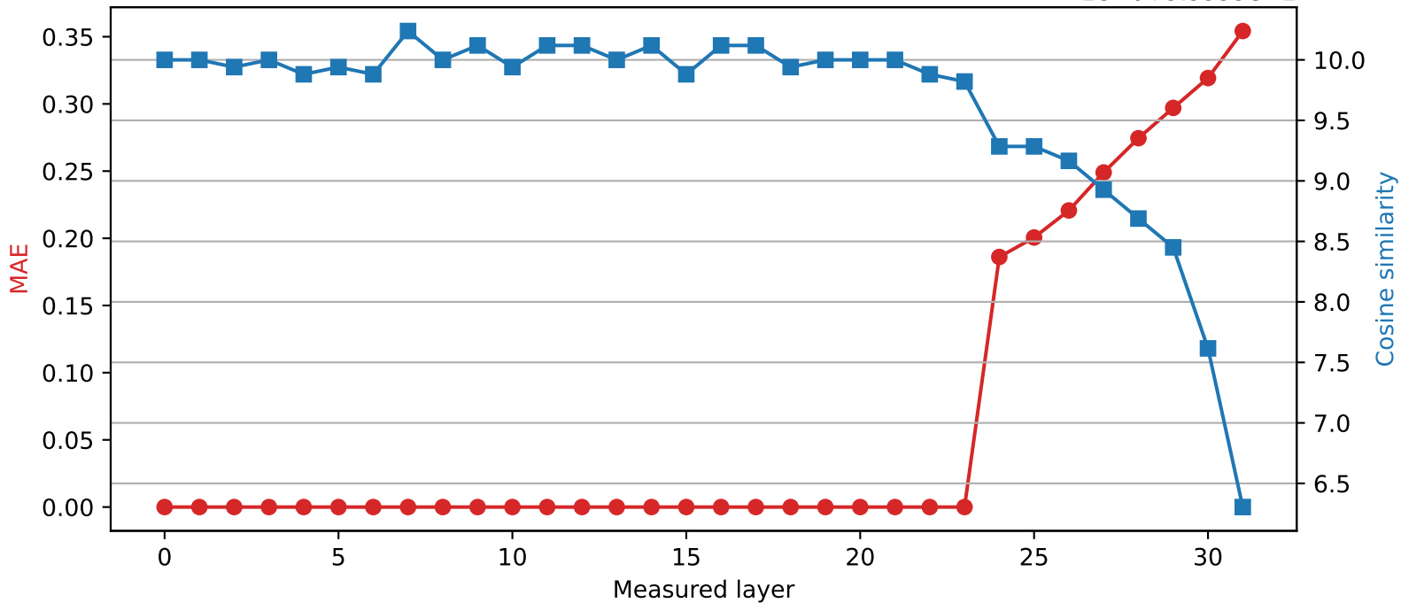
SmolLM2-360M | Quantized layer 23 | float64 \rightarrow int8 1e-6+9.9999e-1
