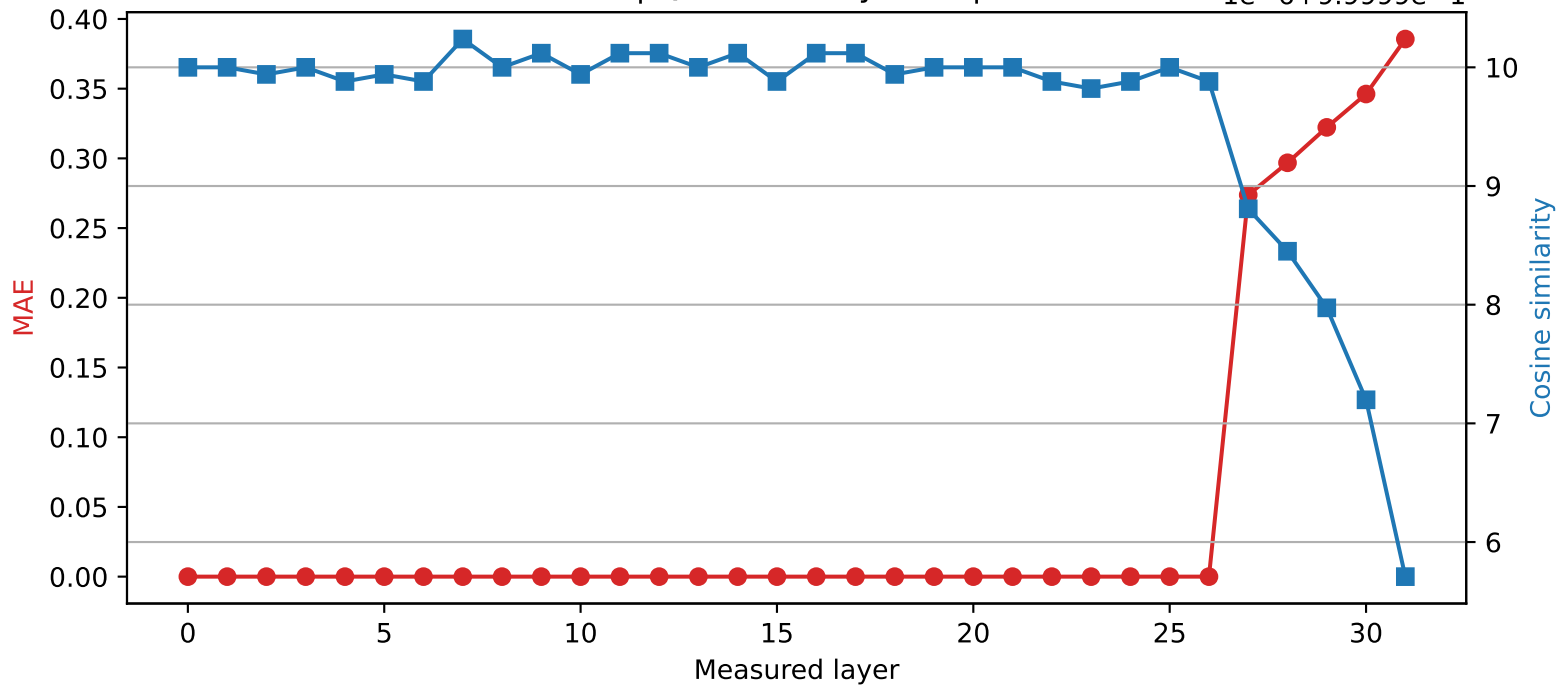
SmolLM2-360M | Quantized layer 26 | float64 → int8 1e-6+9.9999e-1
