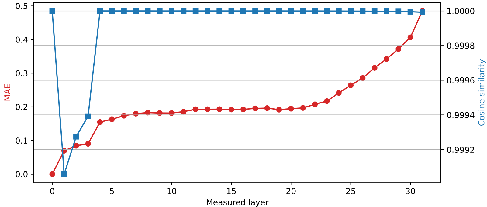
SmolLM2-360M | Quantized layer 0 | float64 \rightarrow int8
