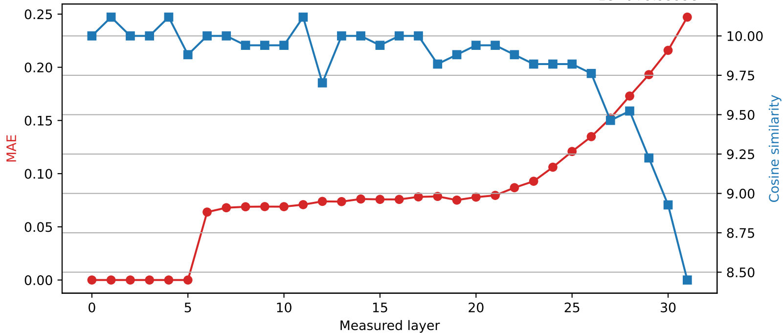
SmolLM2-360M | Quantized layer 5 | float64 \rightarrow int8 1e-6+9.9999e-1
