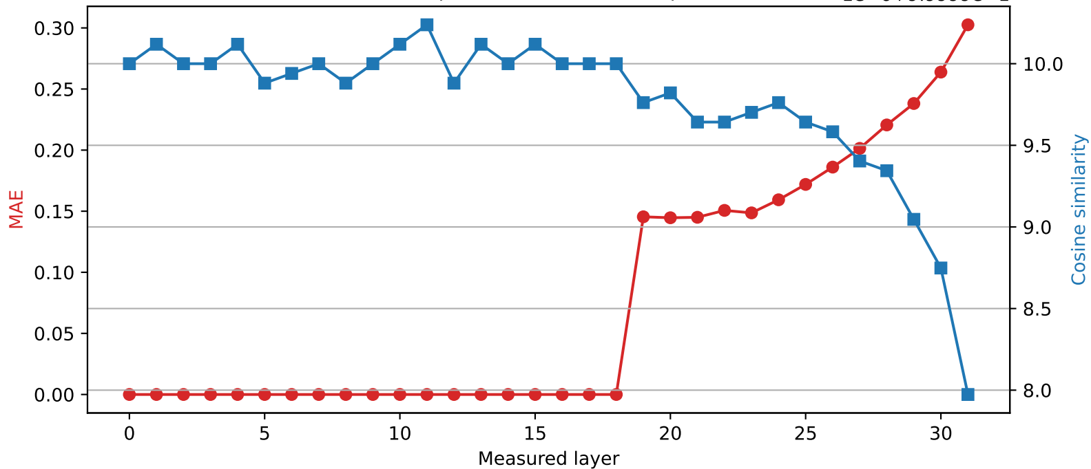
SmolLM2-360M | Quantized layer 18 | float64 \rightarrow int8 1e-6+9.9999e-1
