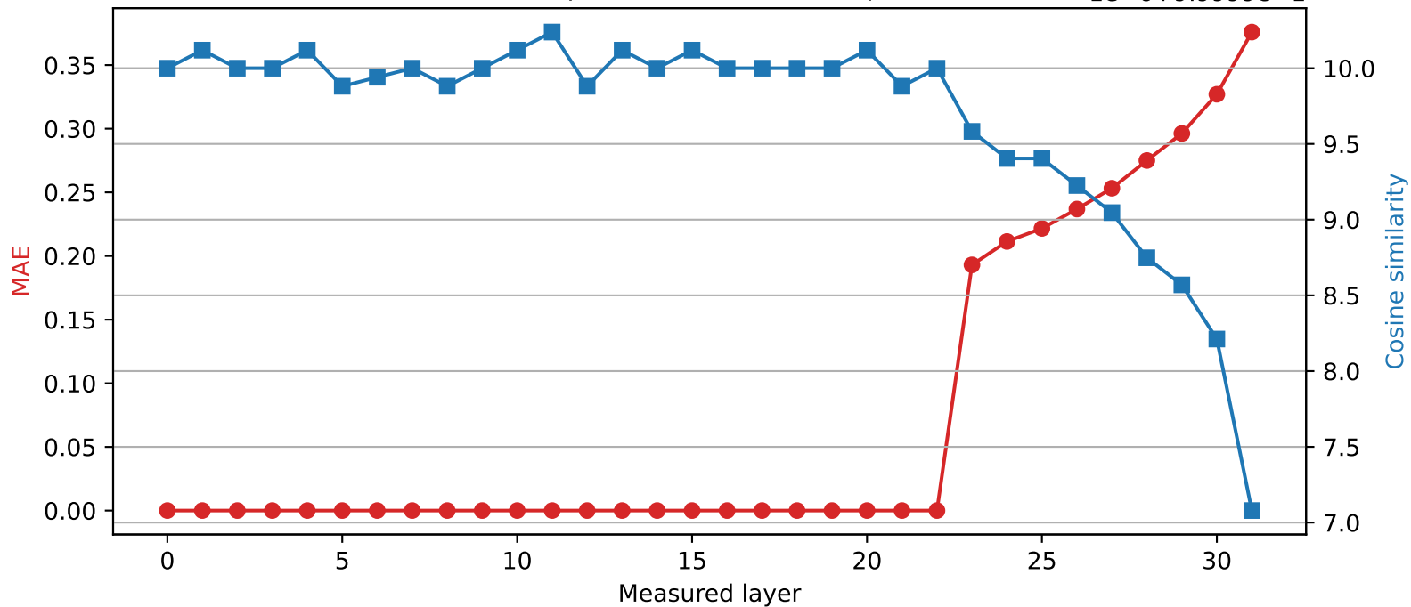
SmolLM2-360M | Quantized layer 22 | float64 \rightarrow int8 1e-6+9.9999e-1
