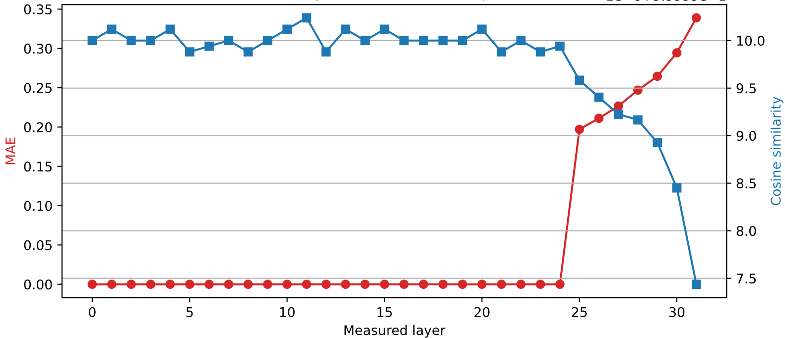
SmolLM2-360M | Quantized layer 24 | float64 \rightarrow int8 1e-6+9.9999e-1
