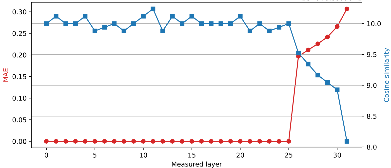
SmolLM2-360M | Quantized layer 25 | float64 \rightarrow int8 1e-6+9.9999e-1
