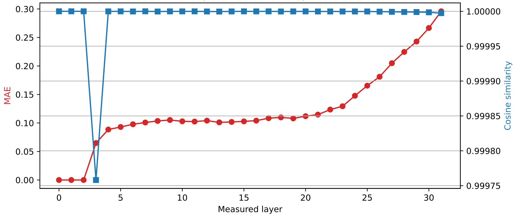
SmolLM2-360M | Quantized layer 2 | float64 → int8
