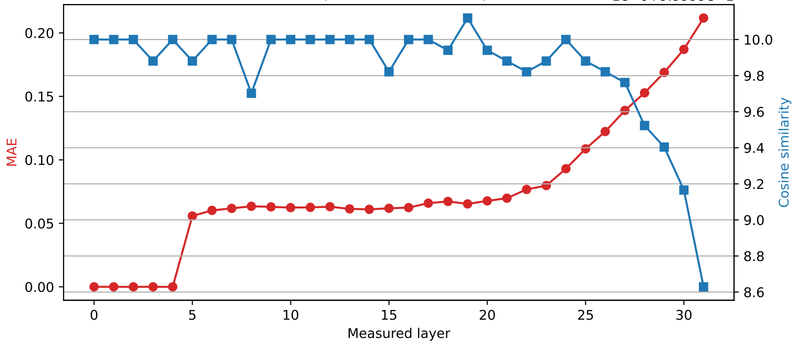
SmolLM2-360M | Quantized layer 4 | float64 → int8 1e-6+9.9999e-1
