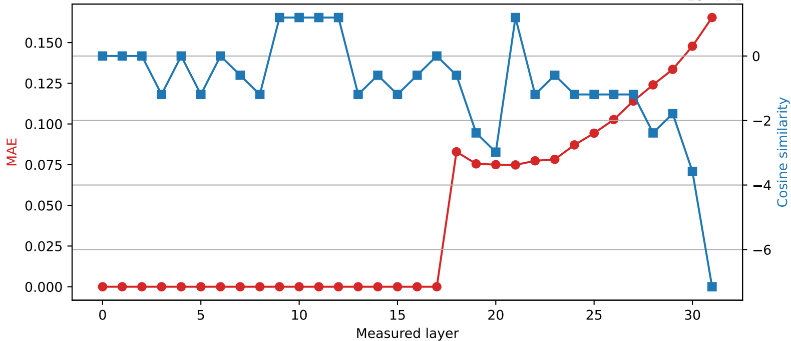
SmolLM2-360M | Quantized layer 17 | float64 → int8
