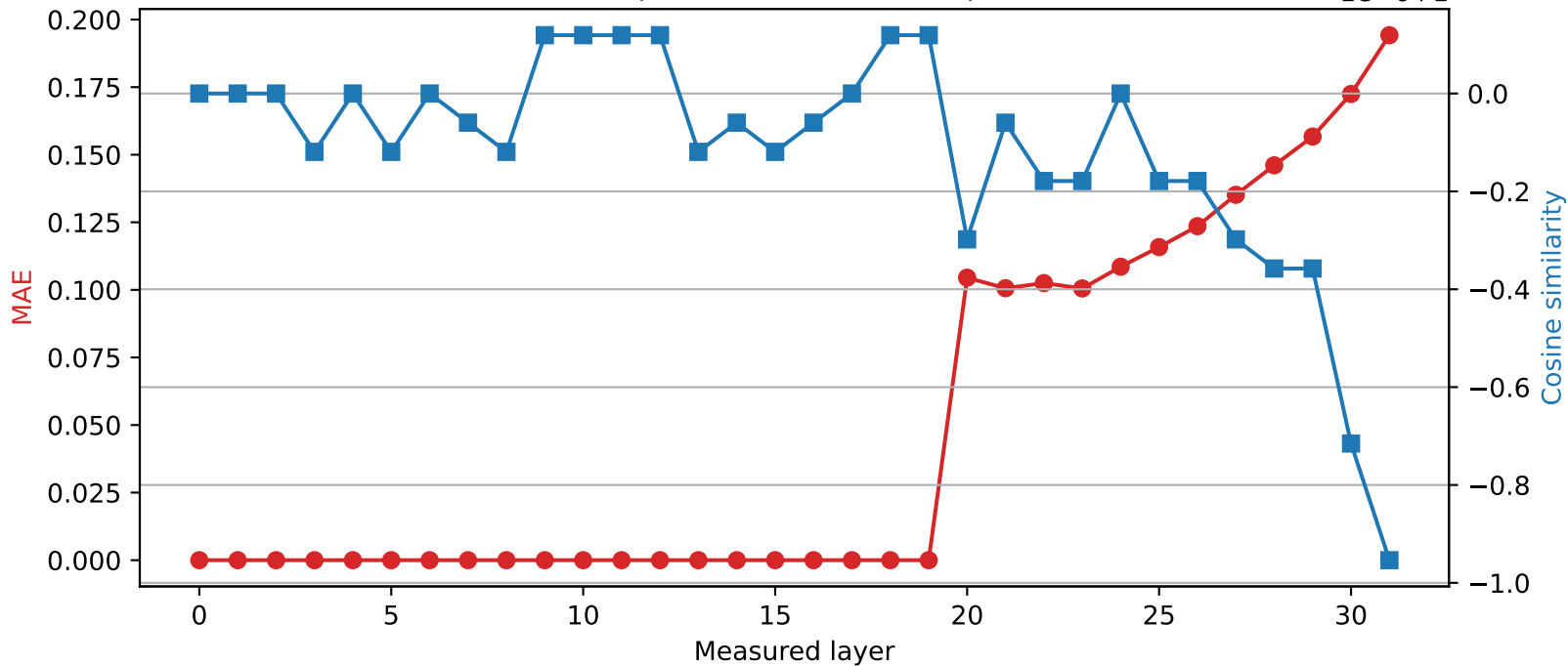
SmolLM2-360M | Quantized layer 19 | float64 → int8
