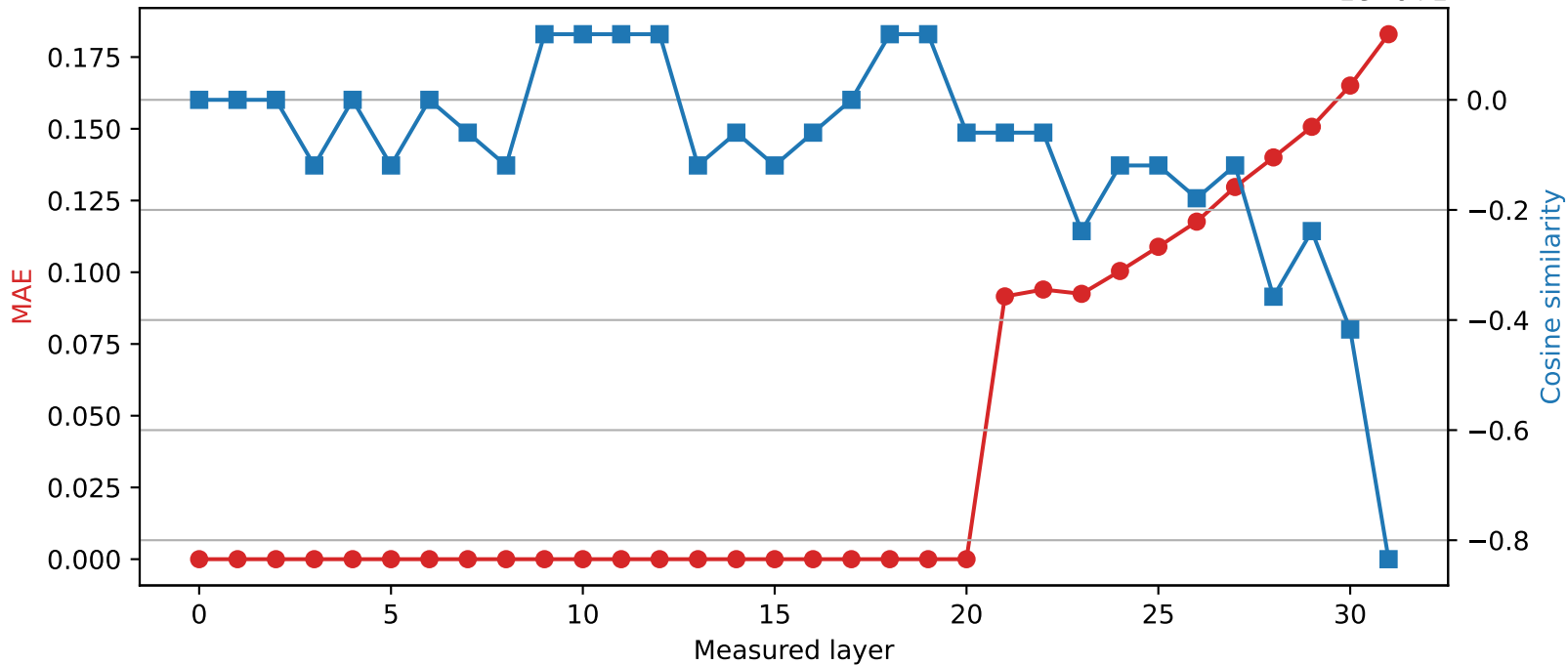
SmolLM2-360M | Quantized layer 20 | float64 → int8
