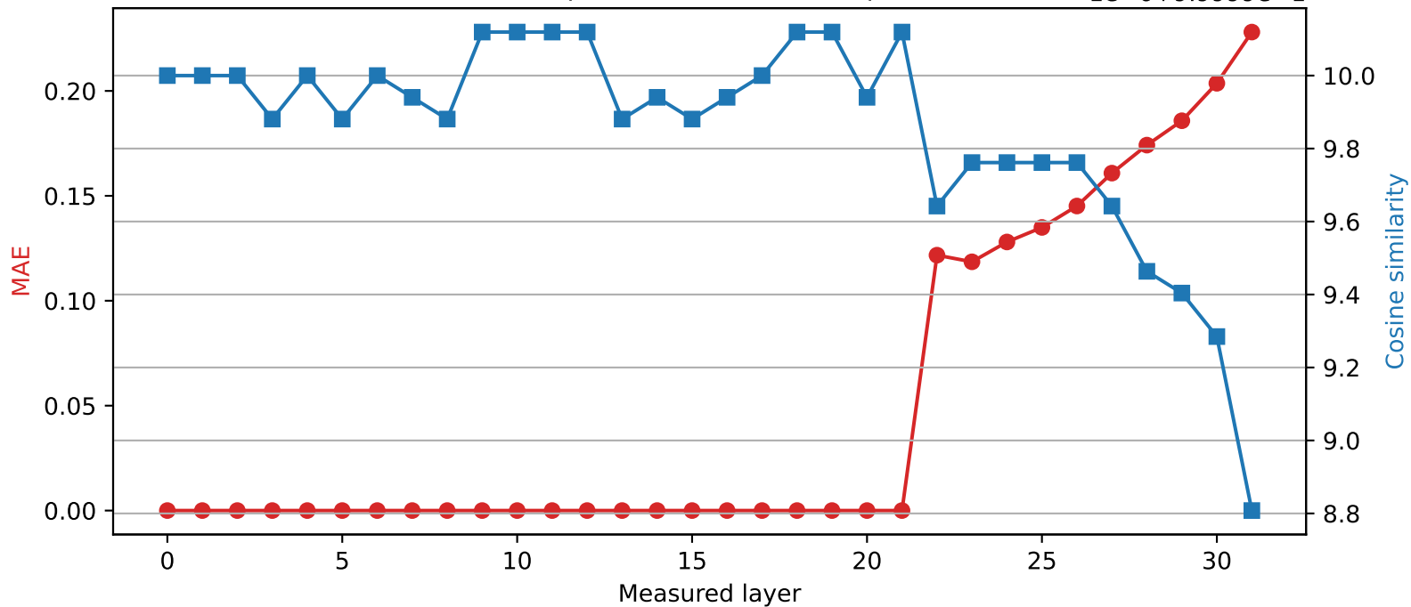
SmolLM2-360M | Quantized layer 21 | float64 \rightarrow int8 1e-6+9.9999e-1
