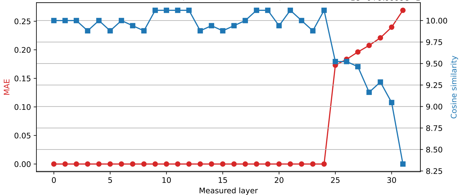
SmolLM2-360M | Quantized layer 24 | float64 → int8 1e-6+9.9999e-1
