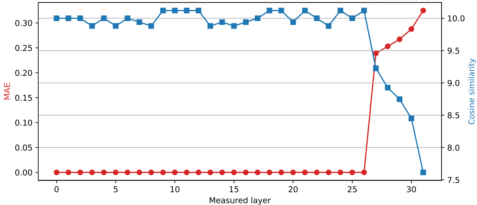
SmolLM2-360M | Quantized layer 26 | float64 \rightarrow int8 1e-6+9.9999e-1
