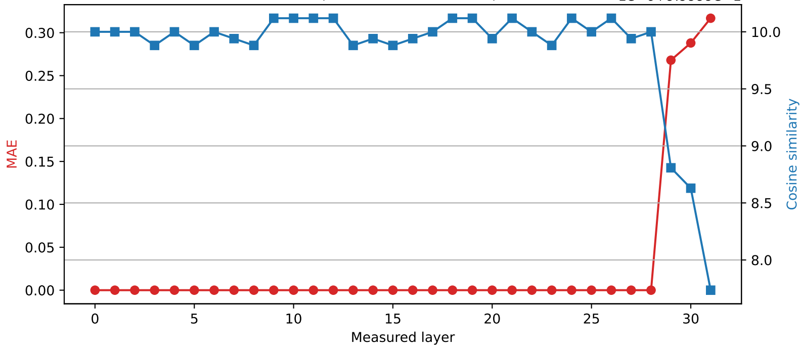
SmolLM2-360M | Quantized layer 28 | float64 \rightarrow int8 1e-6+9.9999e-1
