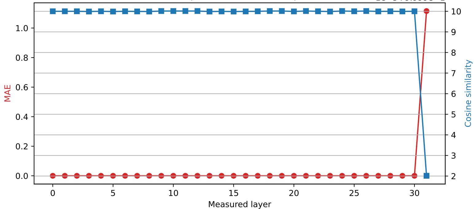
SmolLM2-360M | Quantized layer 30 | float64 → int8
