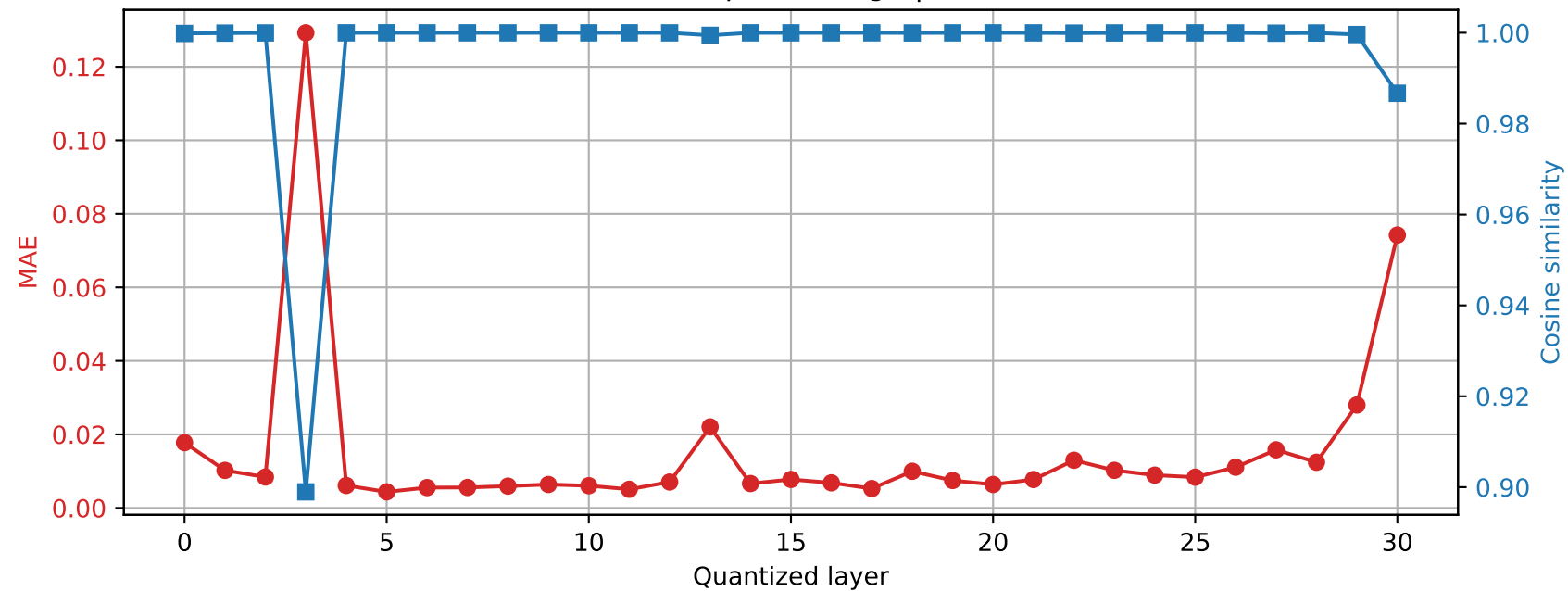
SmolLM2-360M | Prompt 4 Final RMSNorm output damage | float64 → int8
