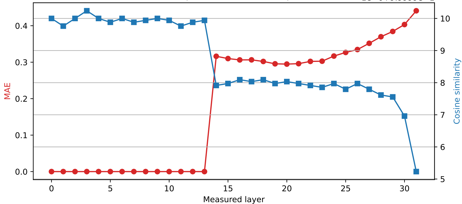
SmolLM2-360M | Quantized layer 13 | float64 \rightarrow int8 1e-6+9.9999e-1
