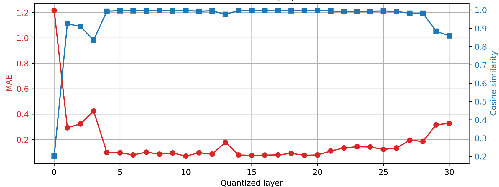
SmolLM2-360M | Prompt 0 Final RMSNorm output damage | float64 \rightarrow int4
