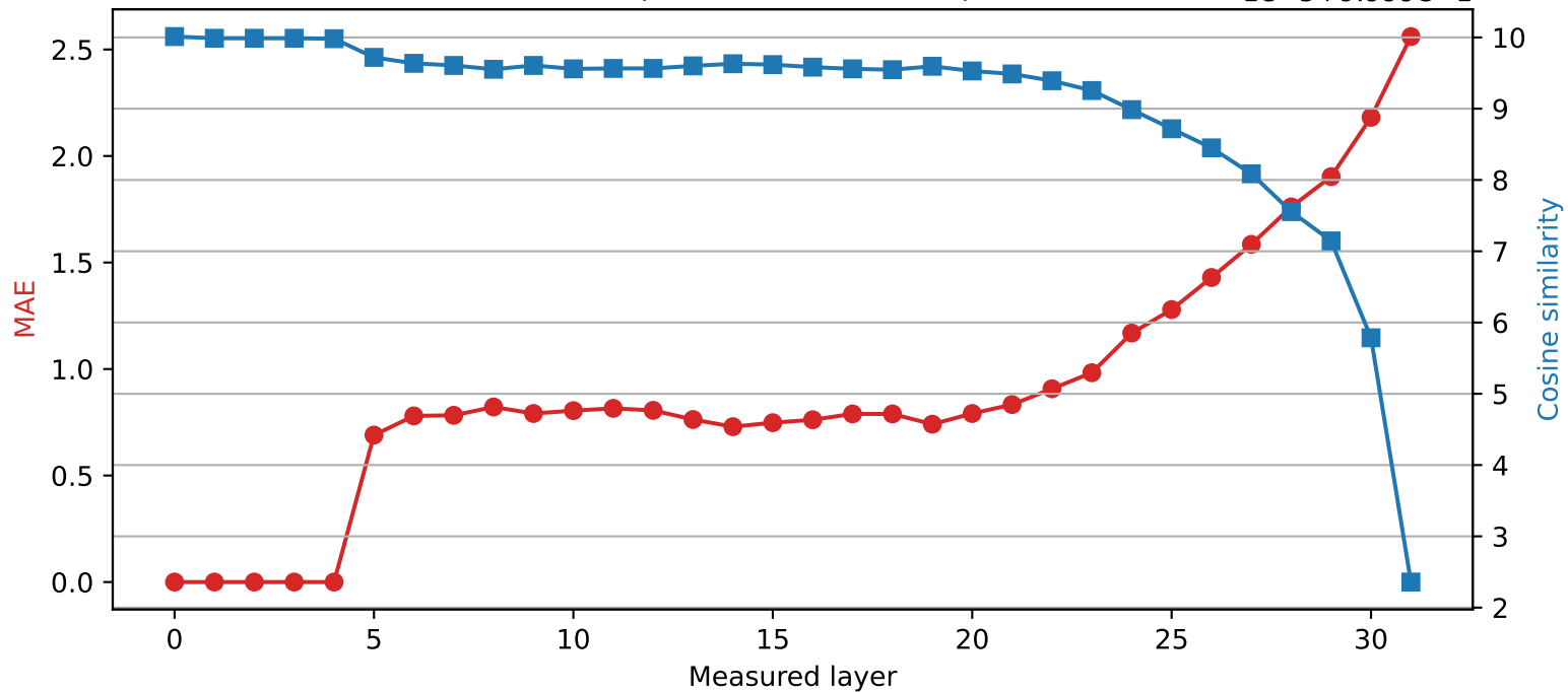
SmolLM2-360M | Quantized layer 4 | float64 → int4
