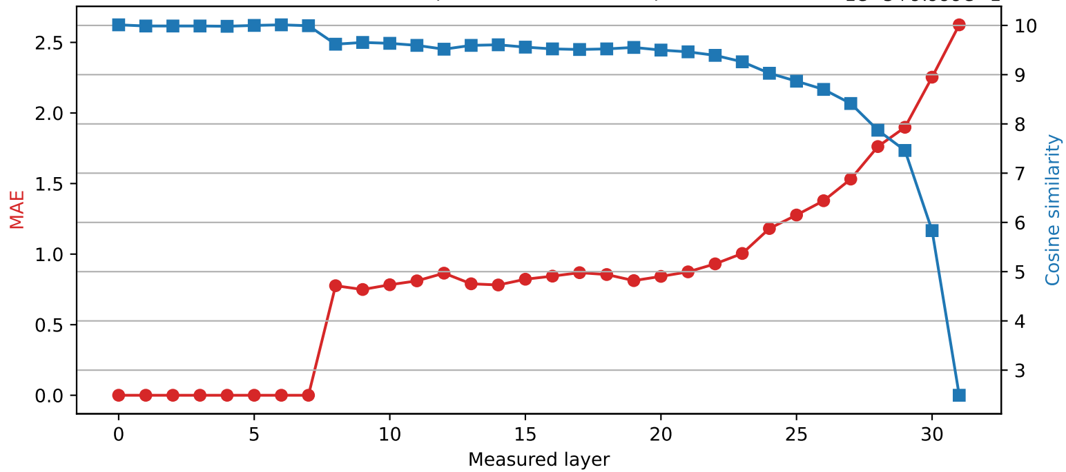
SmolLM2-360M | Quantized layer 7 | float64 → int4
