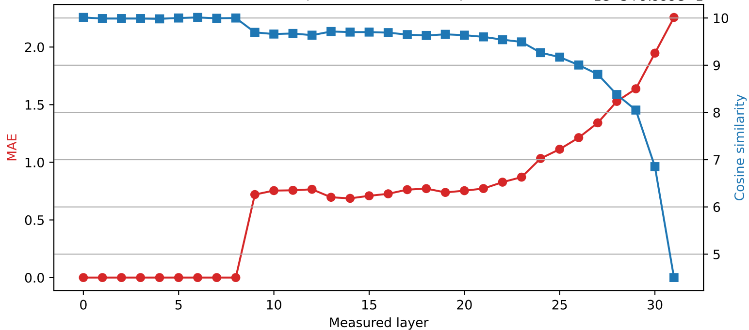
SmolLM2-360M | Quantized layer 8 | float64 → int4
