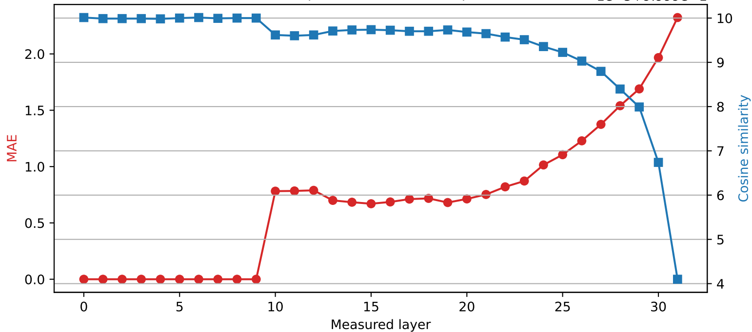
SmolLM2-360M | Quantized layer 9 | float64 → int4
