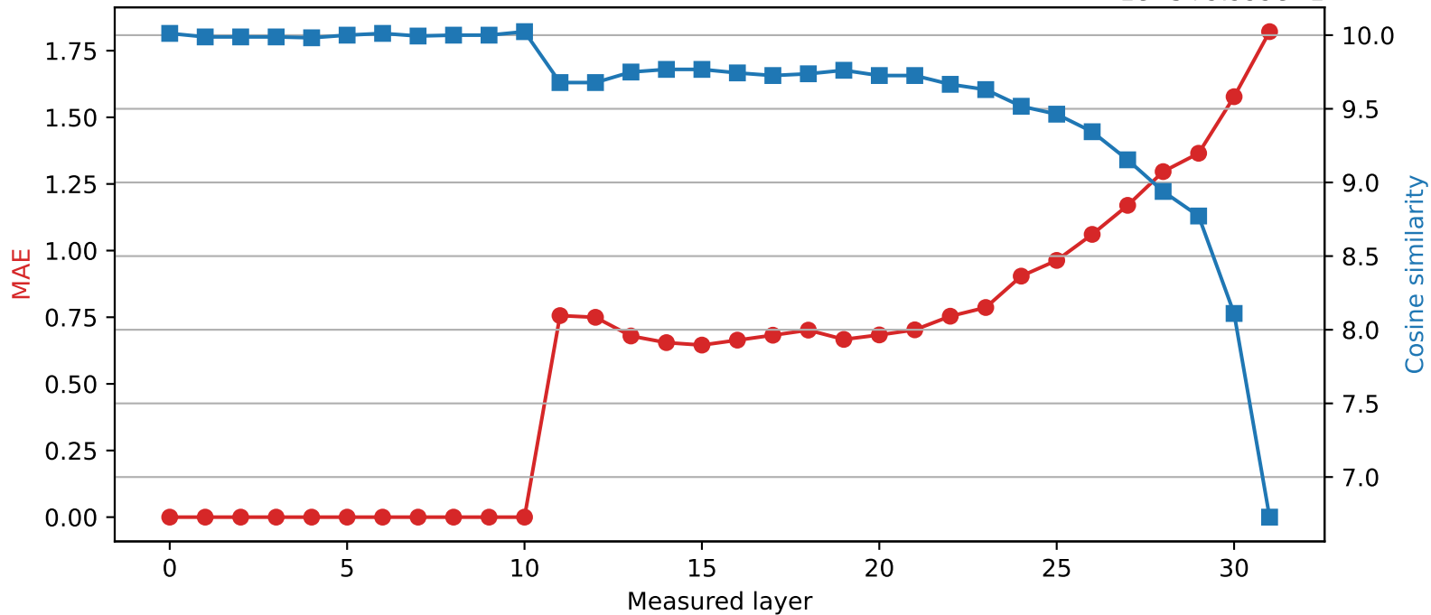
SmolLM2-360M | Quantized layer 10 | float64 → int4 1e-5+9.999e-1
