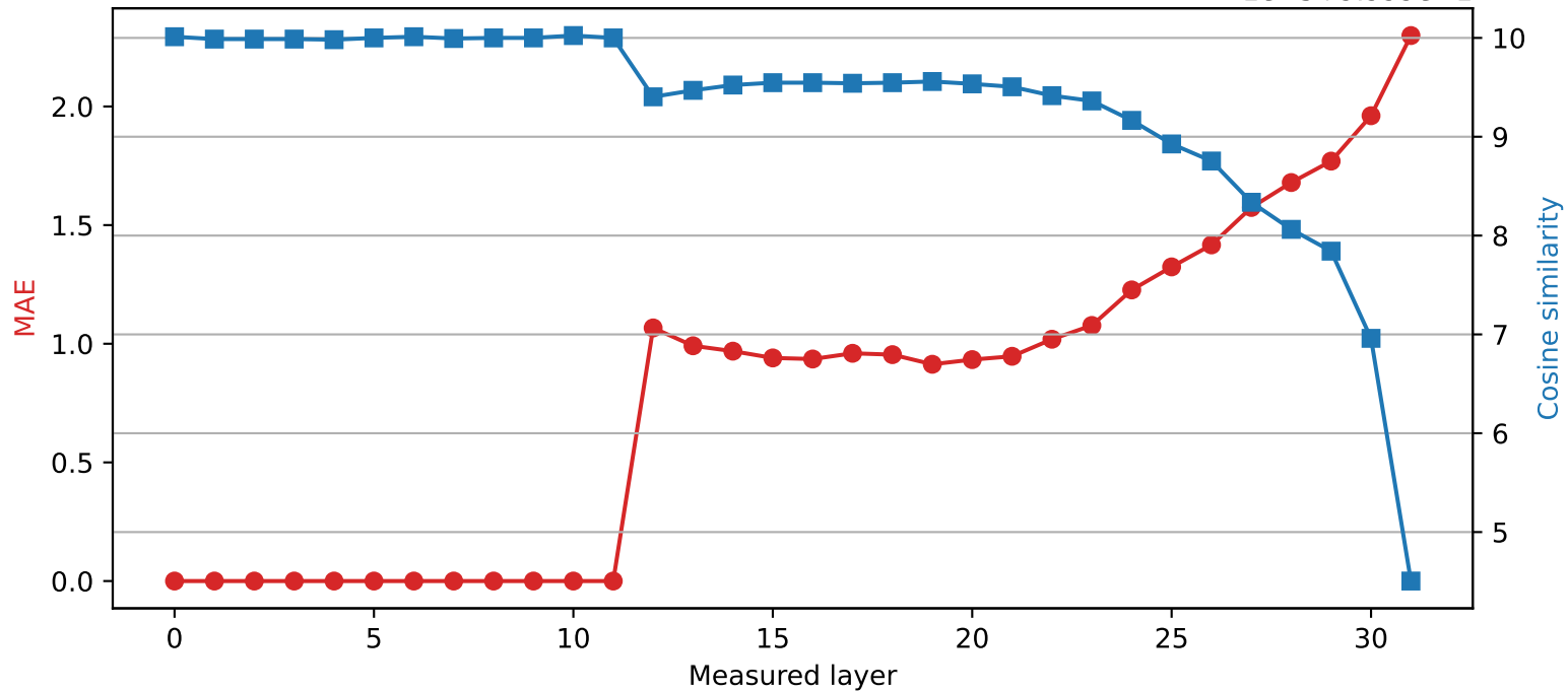
SmolLM2-360M | Quantized layer 11 | float64 → int4 1e-5+9.999e-1
