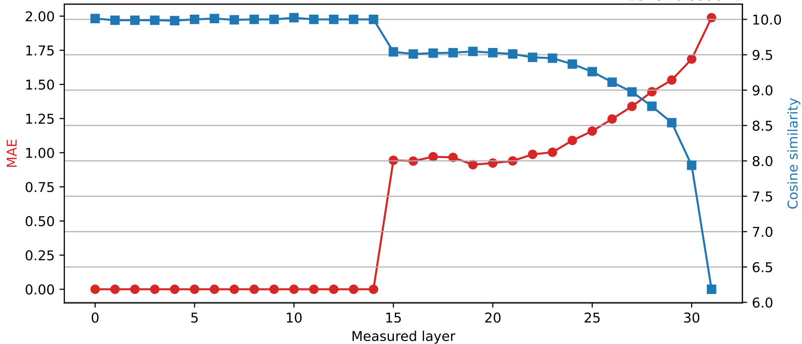
SmolLM2-360M | Quantized layer 14 | float64 → int4 1e-5+9.999e-1
