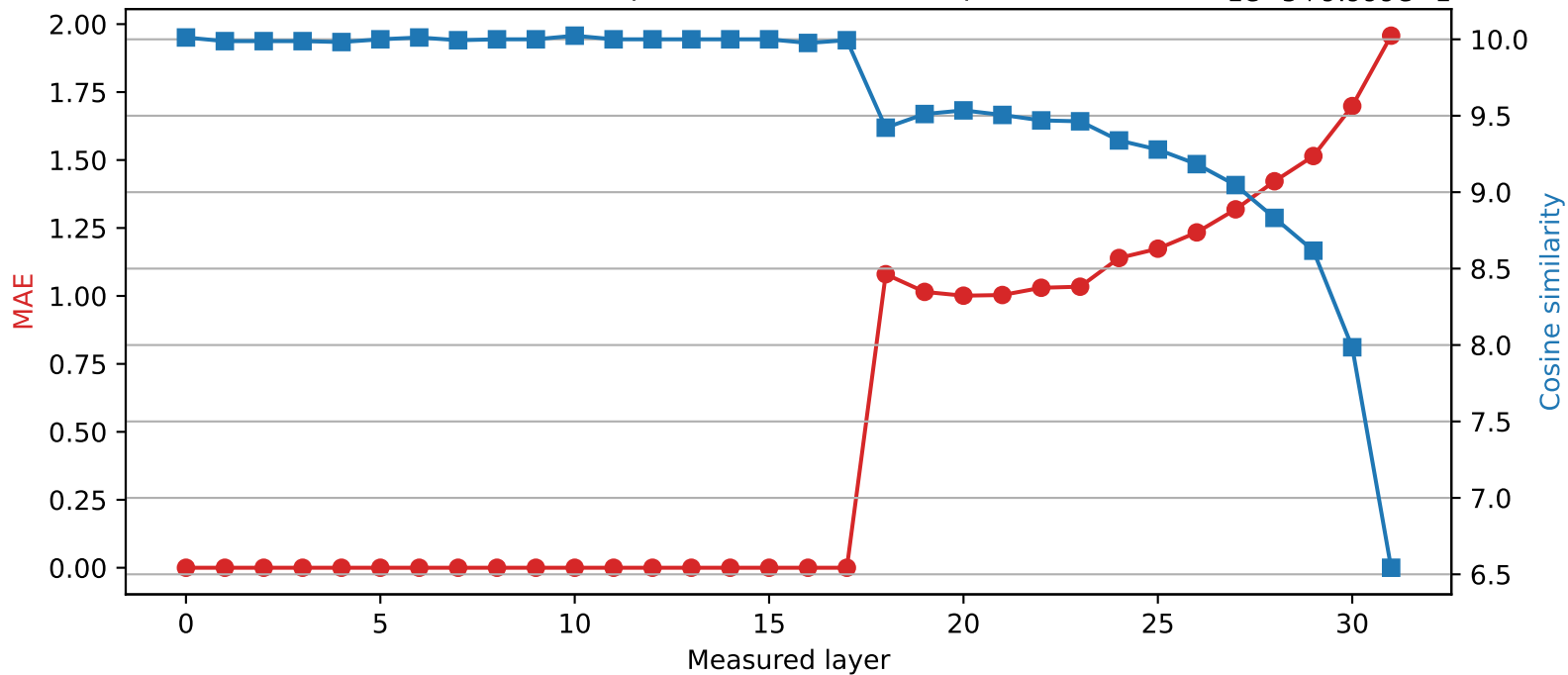
SmolLM2-360M | Quantized layer 17 | float64 → int4 1e-5+9.999e-1
