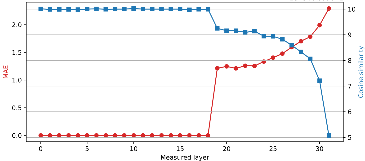
SmolLM2-360M | Quantized layer 18 | float64 → int4 1e-5+9.999e-1
