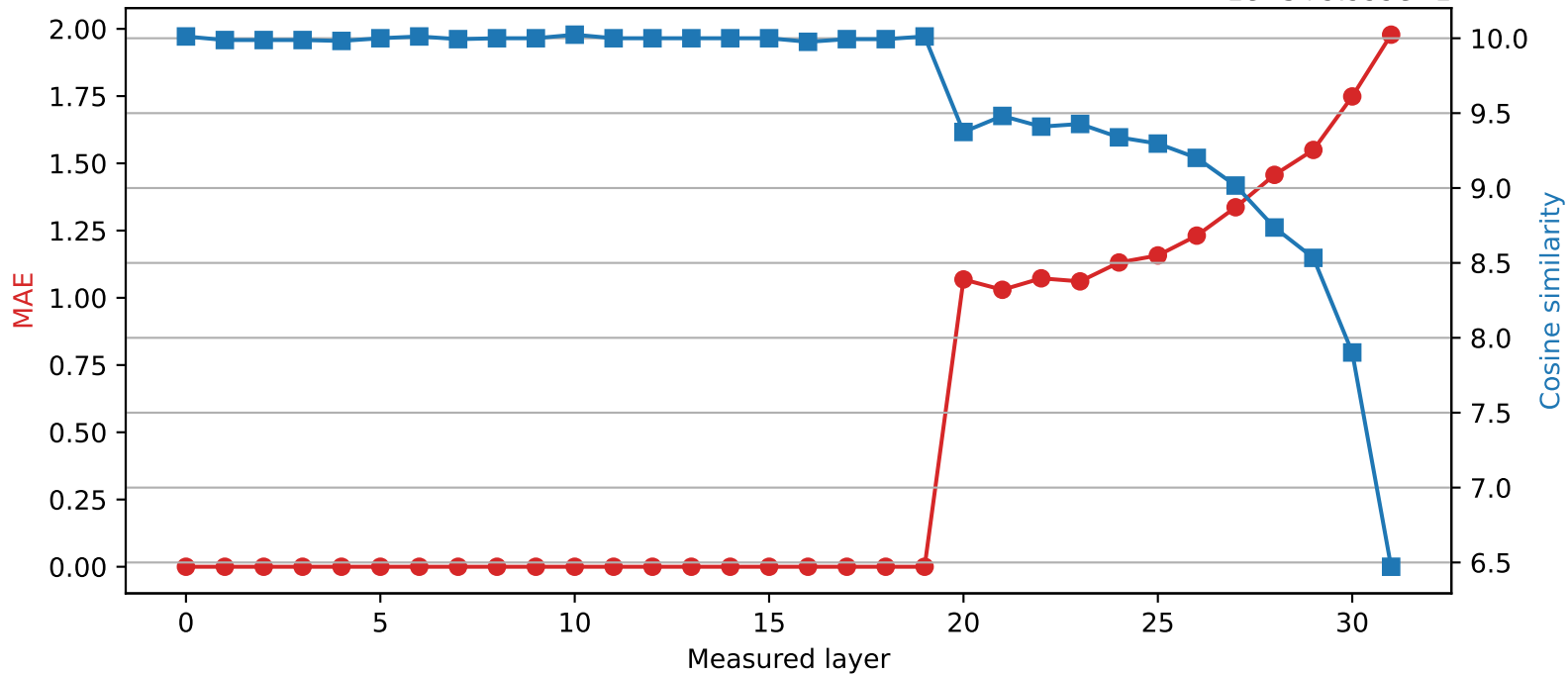
SmolLM2-360M | Quantized layer 19 | float64 → int4 1e-5+9.999e-1
