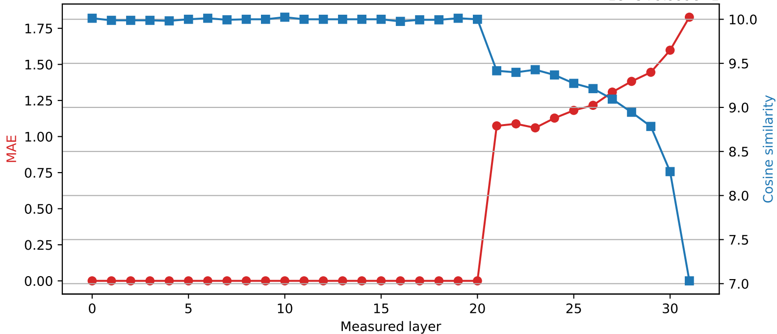
SmolLM2-360M | Quantized layer 20 | float64 \rightarrow int4 1e-5+9.999e-1
