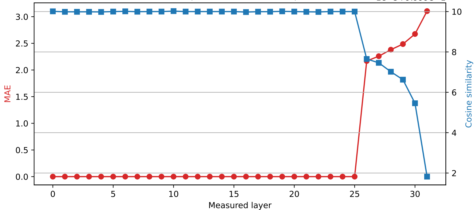
SmolLM2-360M | Quantized layer 25 | float64 → int4 1e-5+9.999e-1
