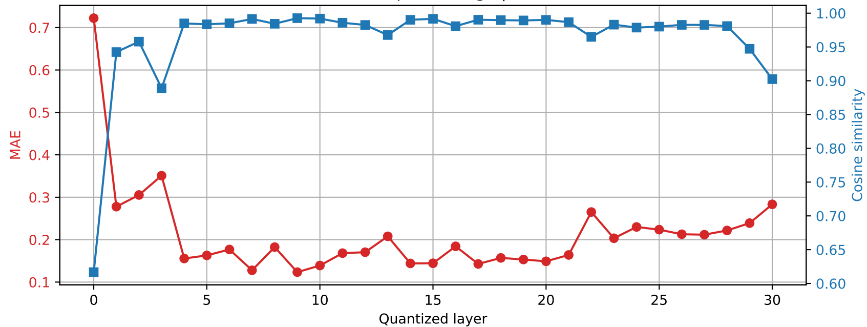
SmolLM2-360M | Prompt 1 Final RMSNorm output damage | float64 → int4
