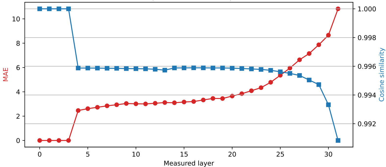
SmolLM2-360M | Quantized layer 3 | float64 → int4
