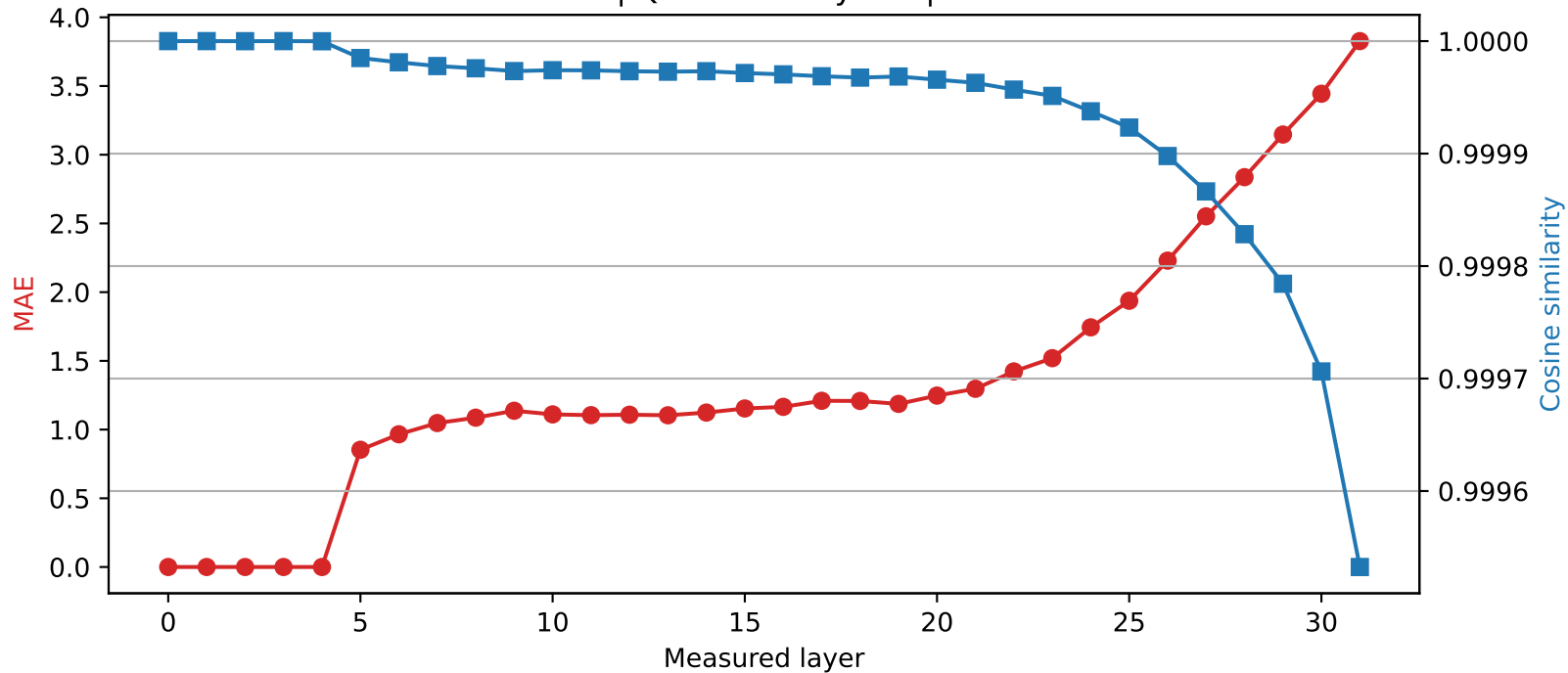
SmolLM2-360M | Quantized layer 4 | float64 → int4
