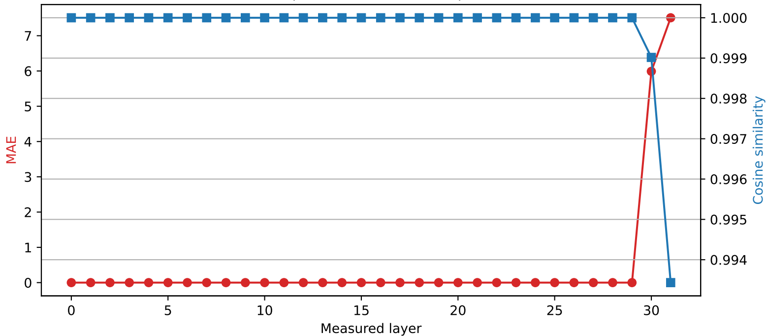
SmolLM2-360M | Quantized layer 29 | float64 → int4
