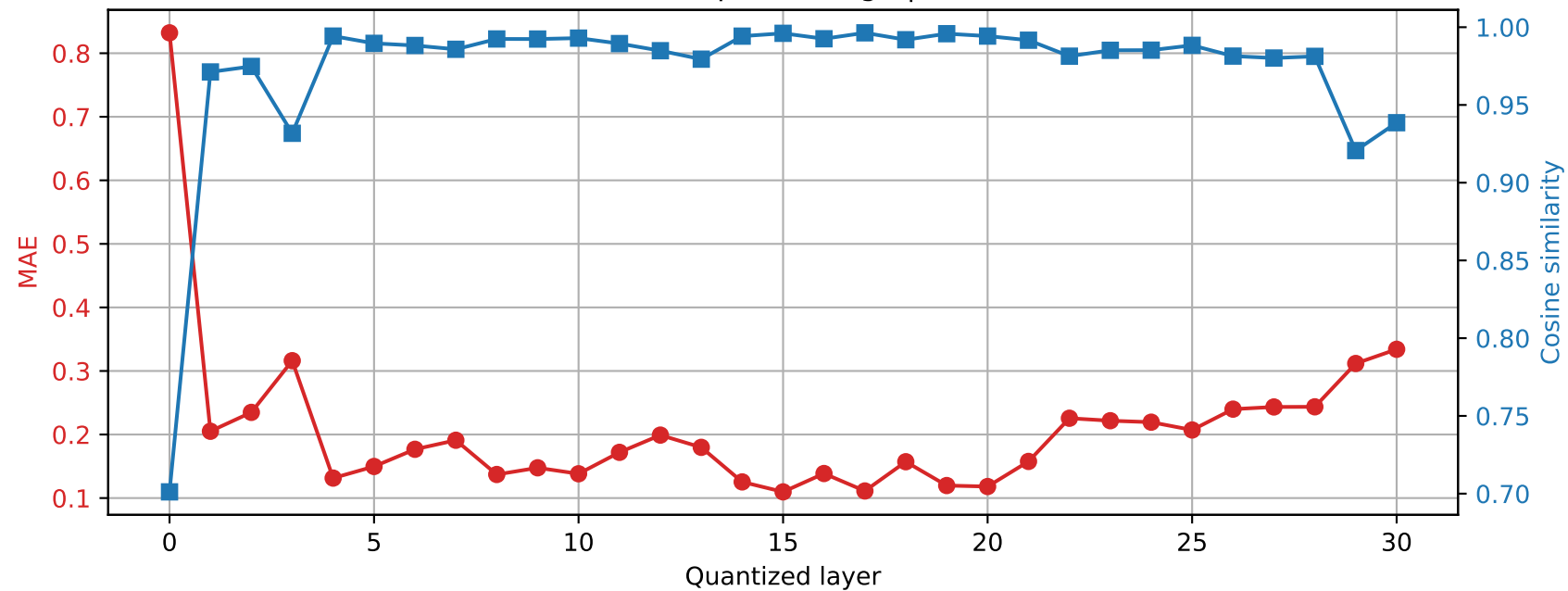
SmolLM2-360M | Prompt 2 Final RMSNorm output damage | float64 → int4
