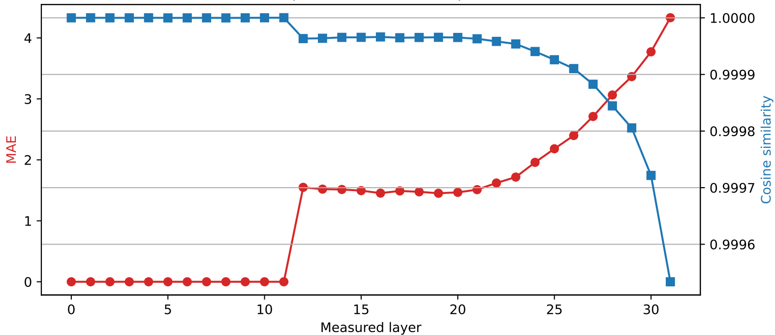
SmolLM2-360M | Quantized layer 11 | float64 → int4
