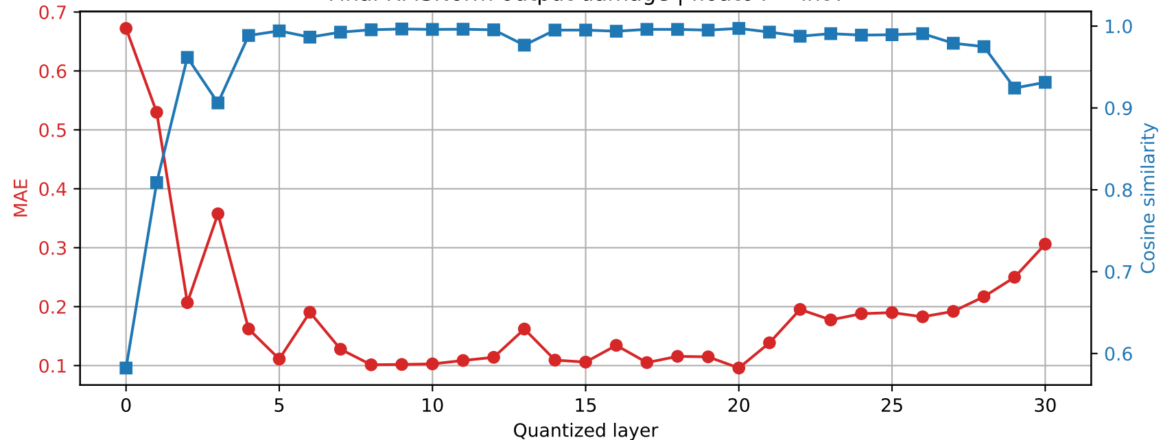
SmolLM2-360M | Prompt 3 Final RMSNorm output damage | float64 \rightarrow int4
