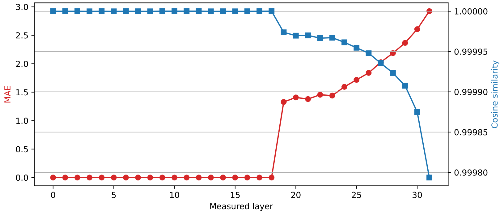
SmolLM2-360M | Quantized layer 18 | float64 → int4
