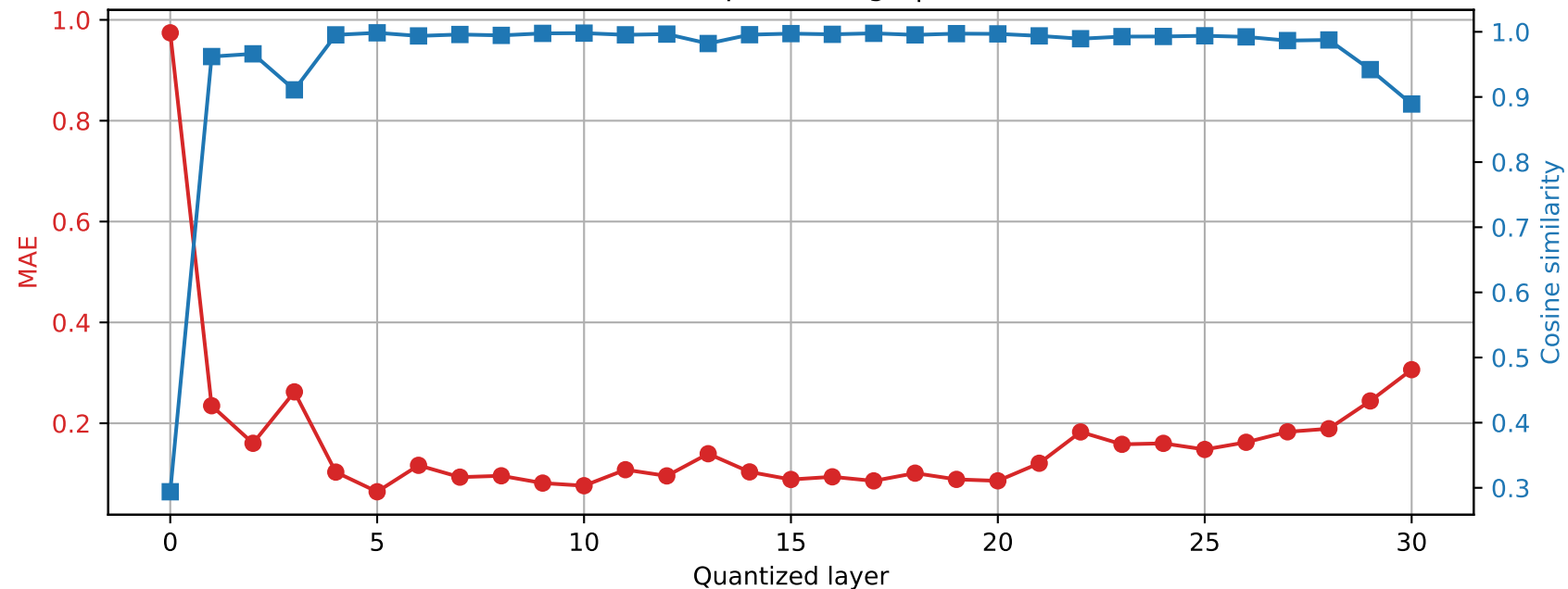
SmolLM2-360M | Prompt 4 Final RMSNorm output damage | float64 \rightarrow int4
