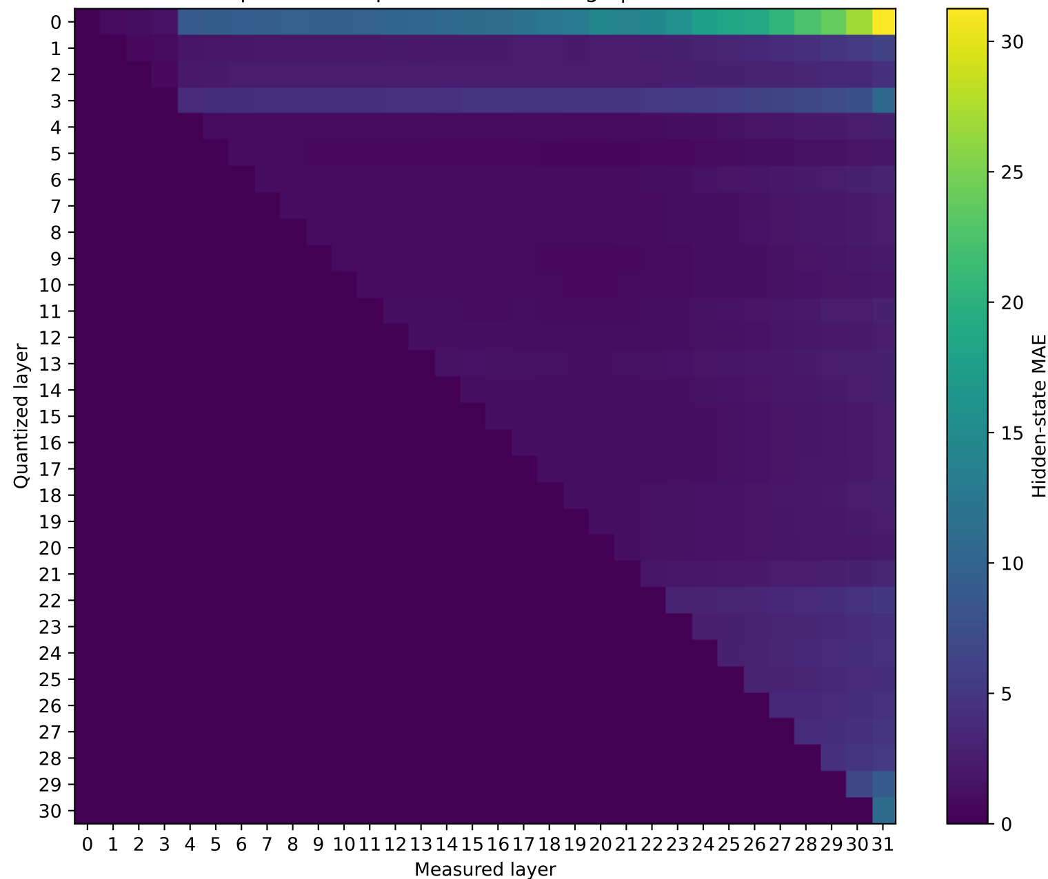
SmolLM2-360M Prompt 4: MAE representation damage | float64 → int4
