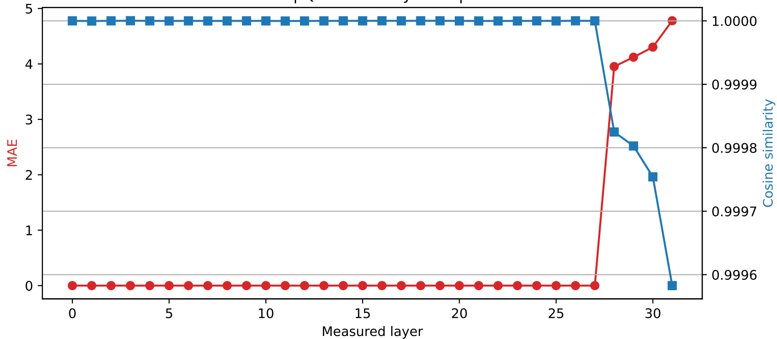
SmolLM2-360M | Quantized layer 27 | float64 → int4
