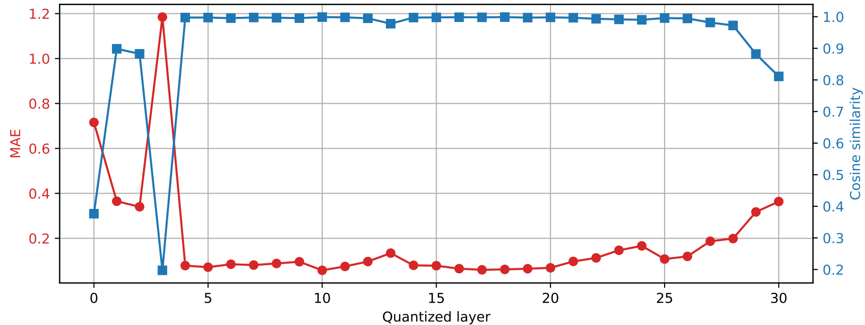
SmolLM2-360M | Prompt 0 Final RMSNorm output damage | float64 \rightarrow int2
