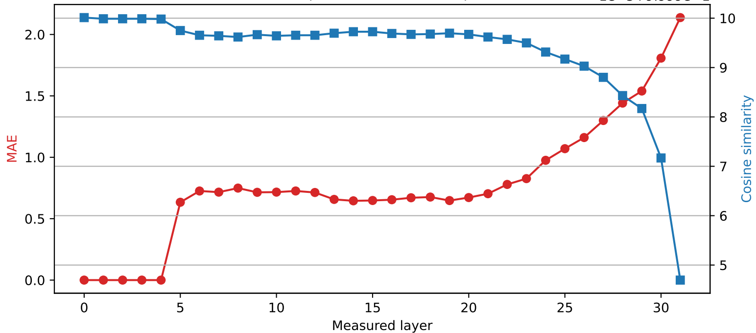
SmolLM2-360M | Quantized layer 4 | float64 → int2
