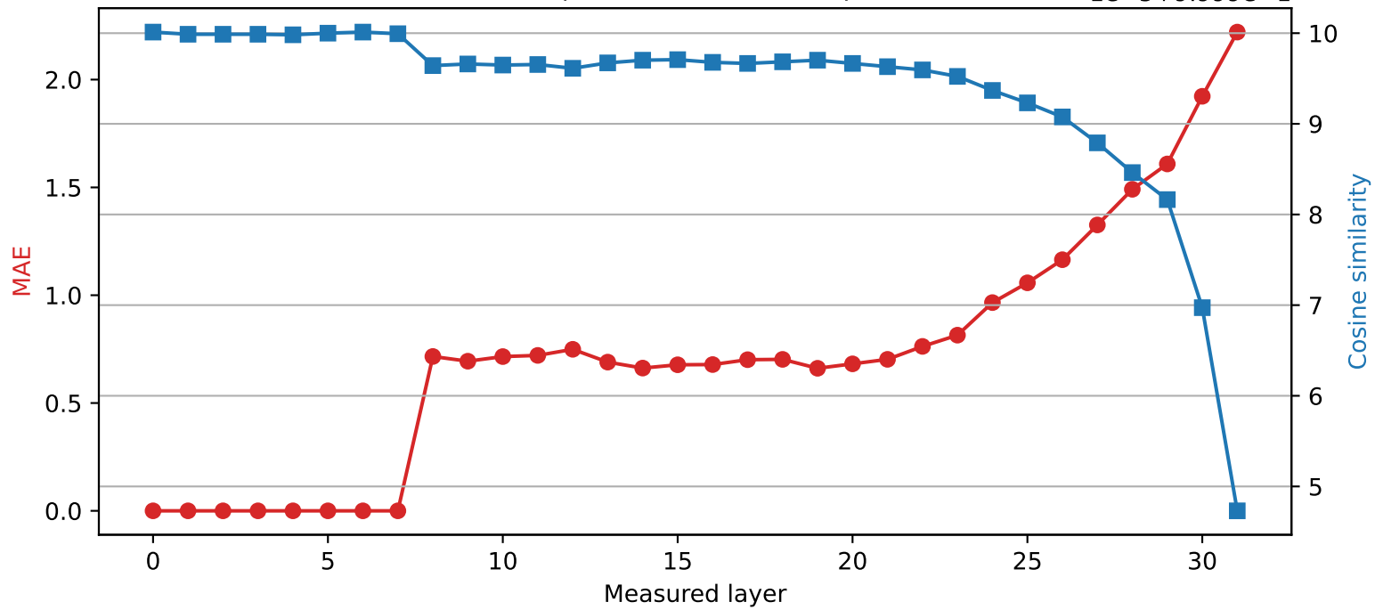
SmolLM2-360M | Quantized layer 7 | float64 → int2
