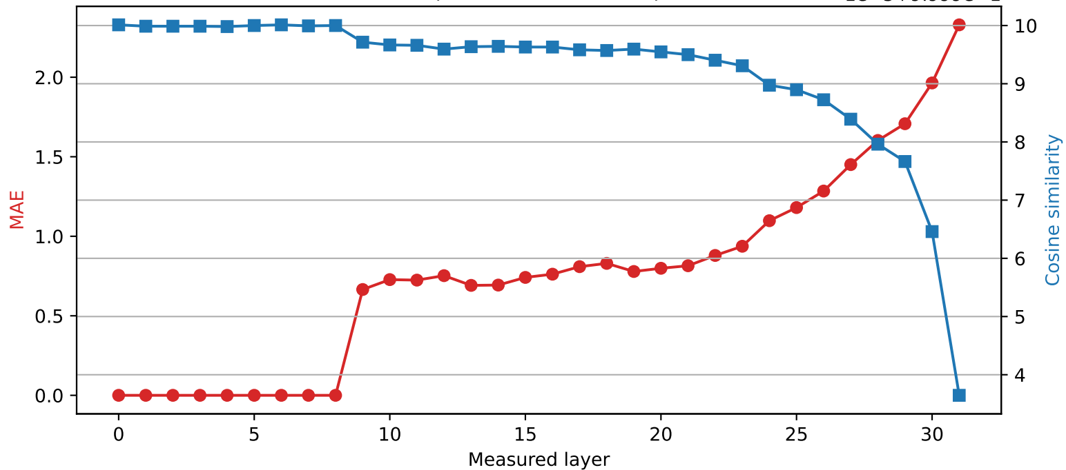
SmolLM2-360M | Quantized layer 8 | float64 → int2
