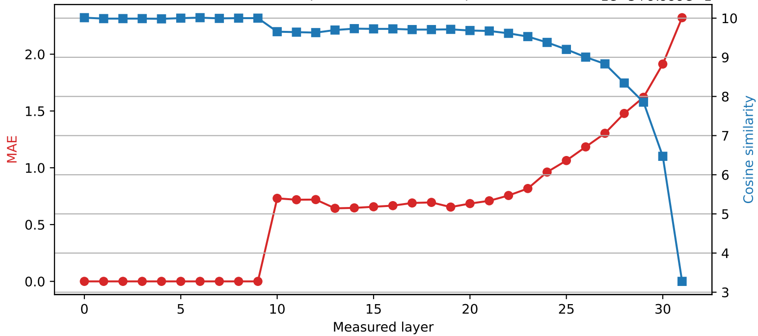
SmolLM2-360M | Quantized layer 9 | float64 → int2
