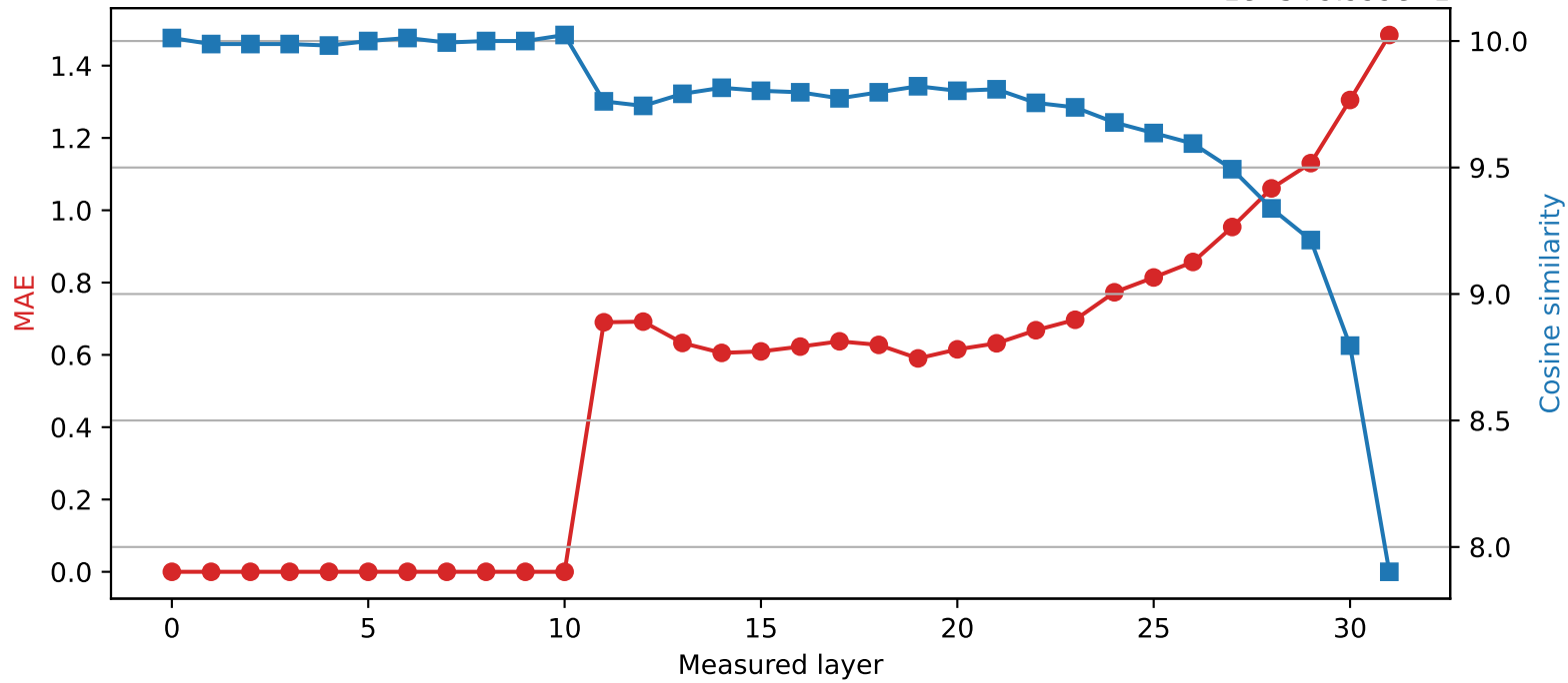
SmolLM2-360M | Quantized layer 10 | float64 → int2 1e-5+9.999e-1
